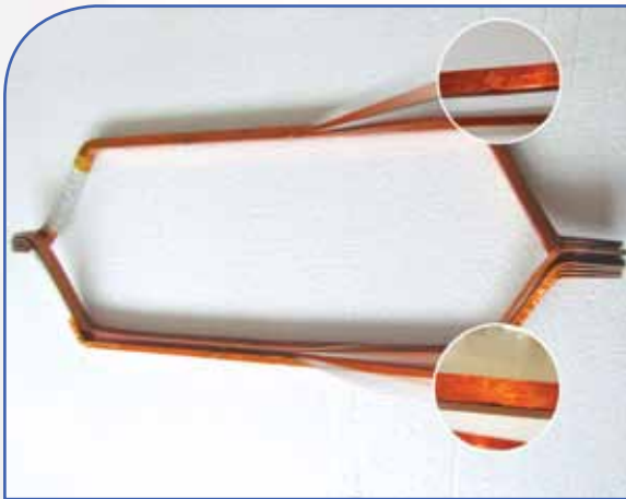
DC TRACTION TRANSPOSED ARMATURE COILS
