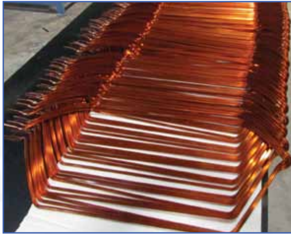
DC TRACTION ARMATURE COILS - LAP WINDING
